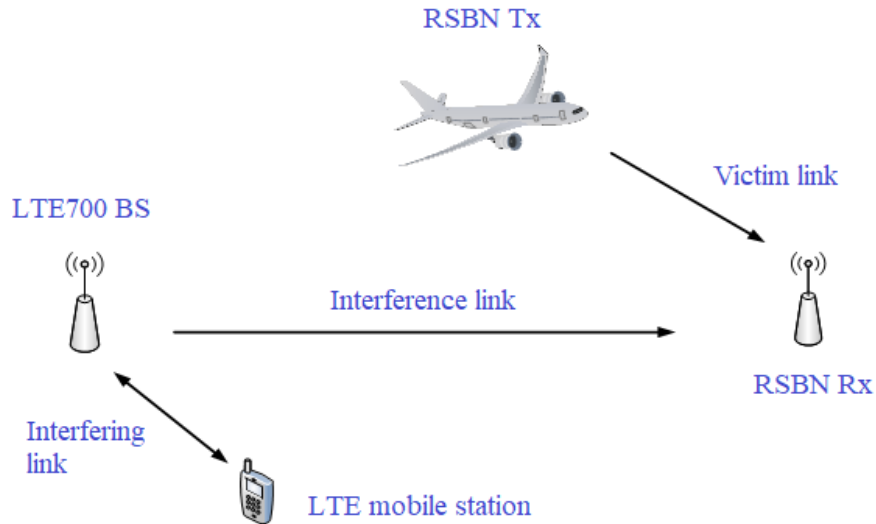
Fig. 3.2. The radio interference scenario for SEAMCAT simulations.
