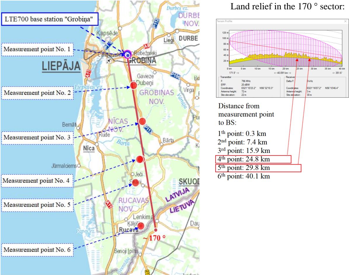
Fig. 3.4. Measurement points of the LTE700 base station signals in the 170° sector on map.
