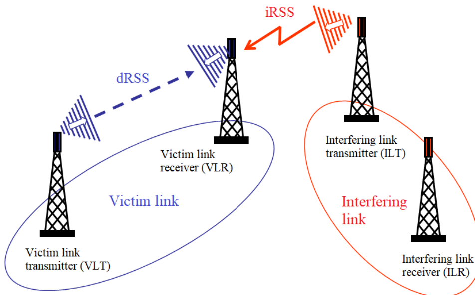
Fig. 2.4. Influenced and interfering network modelling in the SEAMCAT software [18].
