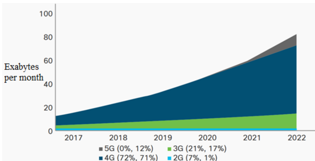
Fig. 1.2. Mobile data traffic forecast by the type of network.
