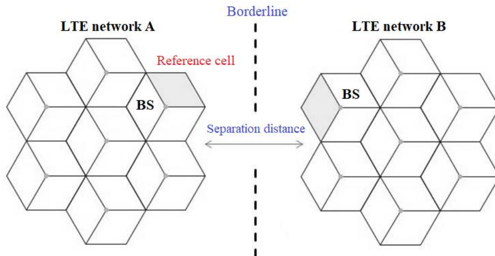
Fig. 3.3. The radio interference scenario for SEAMCAT simulations.
