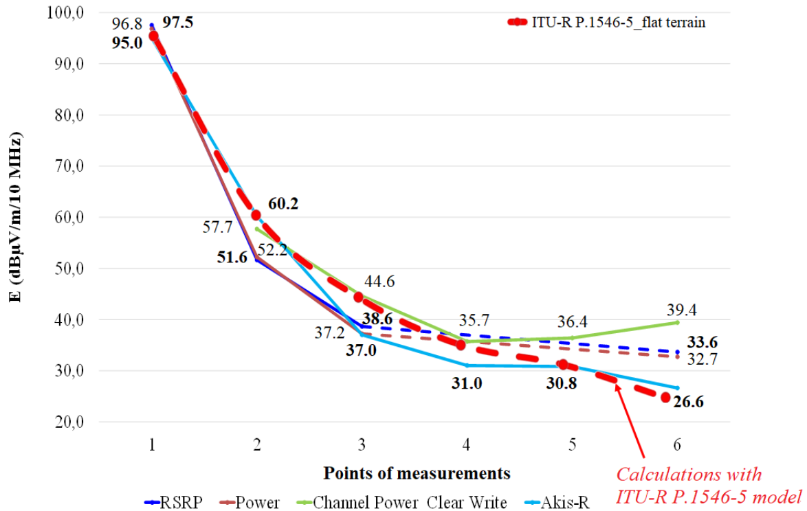
Fig. 3.5. Summary of the measurements of the EMF intensity of the signals transmitted by the LTE700 base station Grobiņa , dBµV/m.
