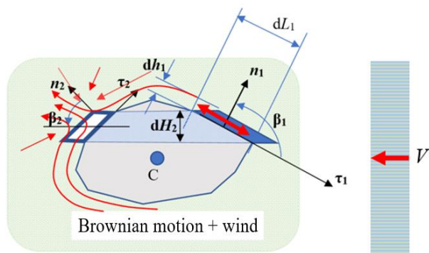
Fig. 2.9. Prismatic model: a) external relative flow over moving-prism in a very low speed airflow; b) interaction of the rectilinear translation (non-rotating) motion body in windless air; c) model of air interactions with stationary prism.
