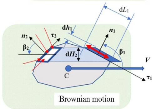
Fig. 2.9. Prismatic model: a) external relative flow over moving-prism in a very low speed airflow; b) interaction of the rectilinear translation (non-rotating) motion body in windless air; c) model of air interactions with stationary prism.
