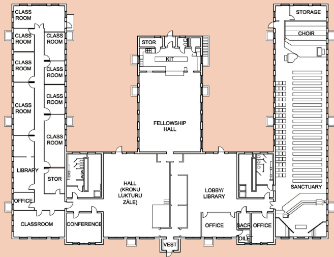
NORTH BUILDING FLOOR PLAN
