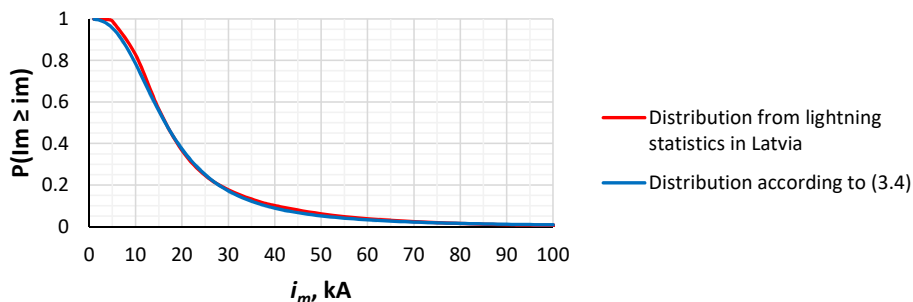
Fig. 3.1. Distribution of lightning peak current in Latvia
