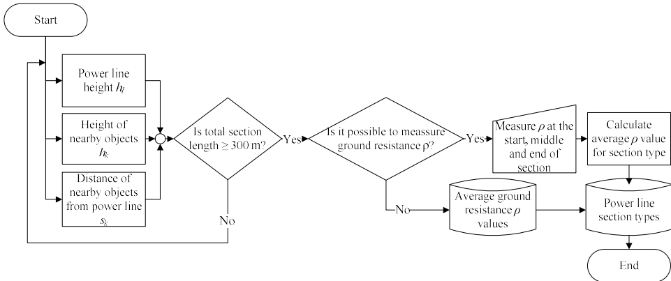
Fig. 5.2. Flowchart of power line section type determination.
