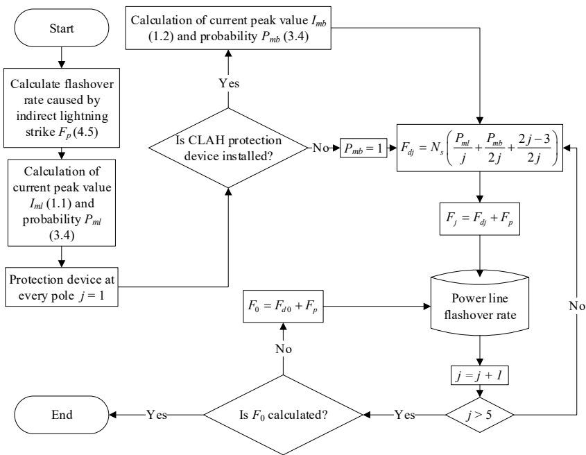
Fig. 5.3. Flowchart of power line flashover rate calculation
