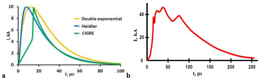
Fig. 2.1. Graphical comparison of lightning current waveshapes: a) lightning current waveshapes of mathematical models 10 kA, 8/20 \mu\text{s} ; b) the first negative lightning return stroke waveshape observed in the nature [20].
