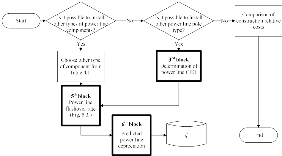
Fig. 5.5. Flowchart of analysis of alternatives.
