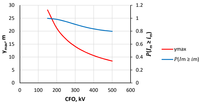
Fig.4.2. The effect of estimated power line CFO on probability of the first stroke peak current I_m that exceeds the value required to cause flashover, and on distance y_{max} to which the power line is subjected to direct and indirect lightning overvoltages.
