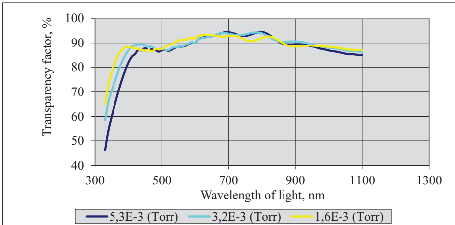
Fig. 4.2. Light transparency curves of three SiO 2 nanolayers.
