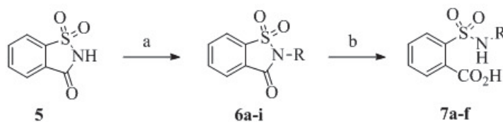
Fig. 7. Synthesis of saccharin derivatives.
