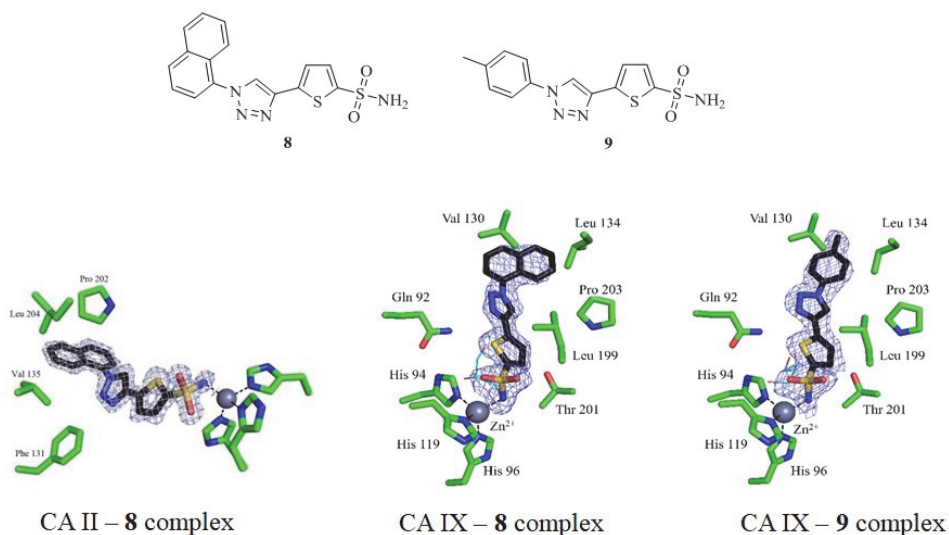
Fig. 8. Structure of compounds 8 and 9 and their co-crystals with CA II and CA IX [15].
