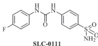
Fig. 1. The structure of CA inhibitor SLC-0111.
