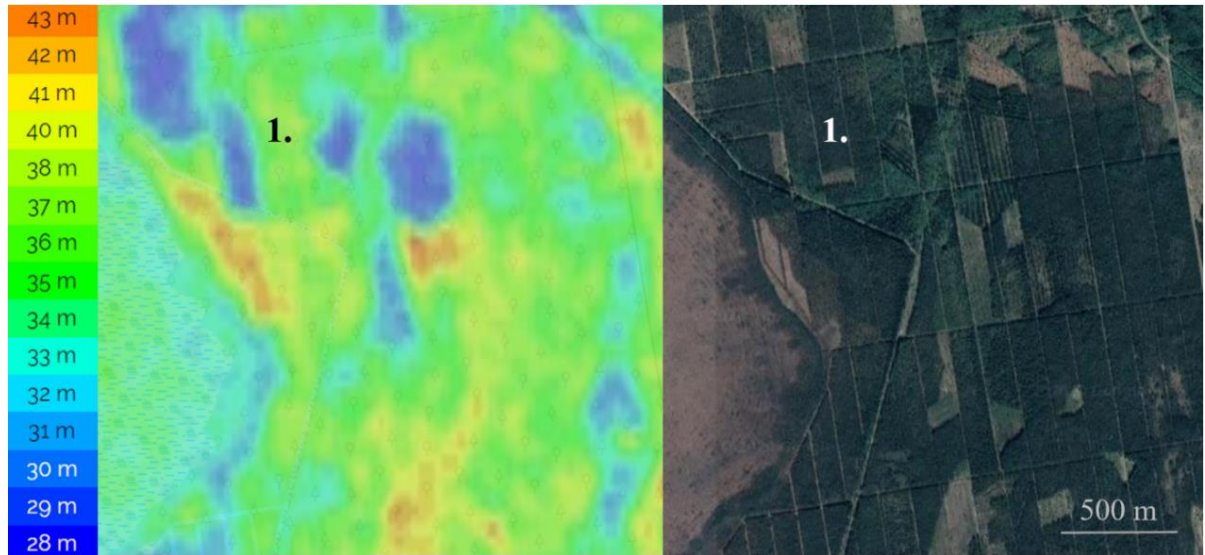
Figure 5. Topographic map and orthographic photograph of the eastern part of Soomaa National Park.
