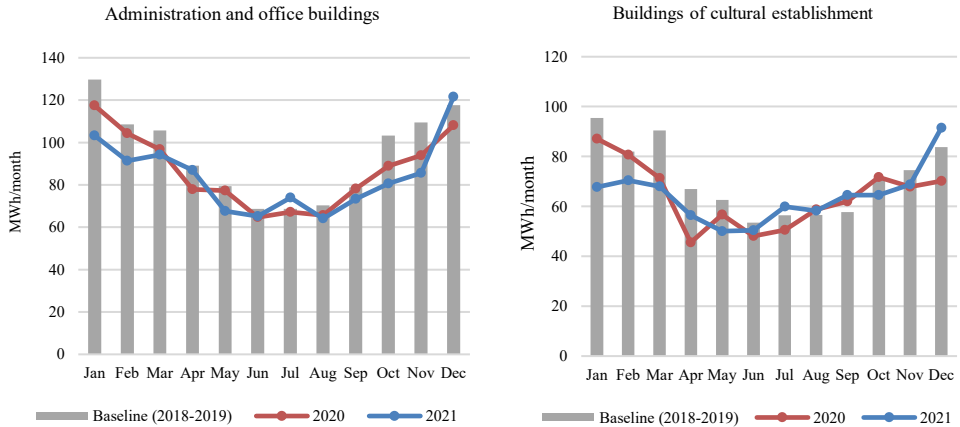
Fig. 9. Electricity consumption in administration and office buildings and in buildings of cultural establishment, MWh/month.
