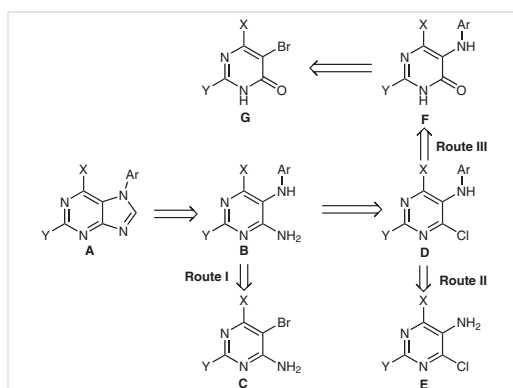
Scheme 1 Retrosynthetic analysis
