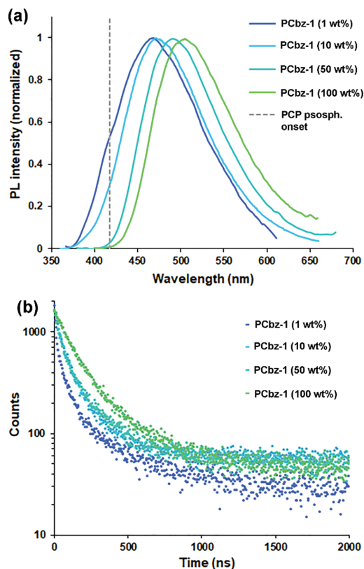
Fig. 6 (a) PL spectra of PCbz-1:PMMA films with different emitter concentrations. Phosphorescence onset of PCP is given to mark the {}^3\text{LE}_A energy level. (b) PL decays of the aforementioned samples.
