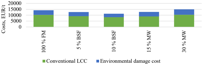
Fig. 3.6. Results of conventional LCC and environmental damage cost results of fish feed alternative.
