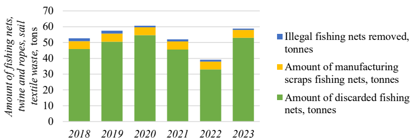
Fig. 3.4. Amount of fishing net waste in Latvia in 2018–2023.
