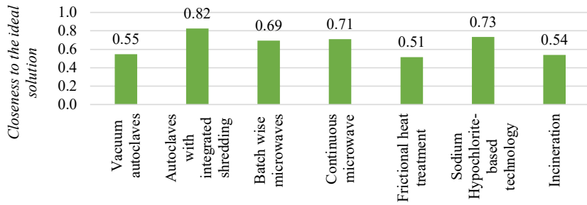
Fig. 3.12. Utility value comparison for iHCW technologies, TOPSIS result.
