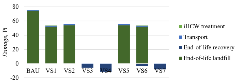
Fig. 3.3. Single score results for BAU and VS1–VS7 (ReCiPe 2016 midpoint (H) method).
