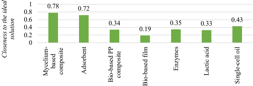
Fig. 3.11. Comparison of utility value for the use of bran by-products, TOPSIS result.
