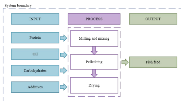
Fig. 3.5. System boundaries for fish feed.
