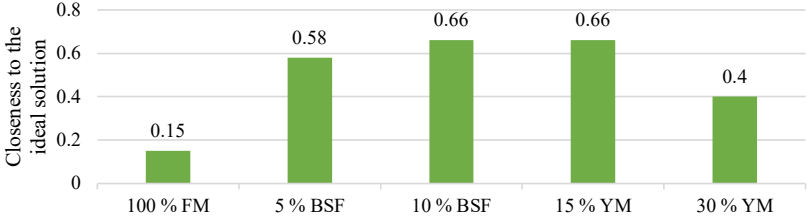
Fig. 3.7. Comparison of the utility value of fish feed composition alternatives, TOPSIS result.
