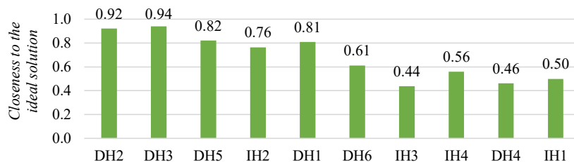
Fig. 3.10. Comparison of the utility value of RES technology in heating supply in municipal, public and residential buildings, TOPSIS result.
