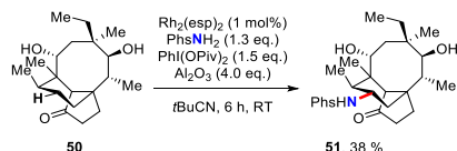
Scheme 13. Intermolecular C-H amination of natural product 50 .
