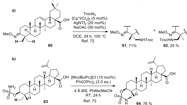
Scheme 15. Previously reported C-H amination examples on the PCT core.
