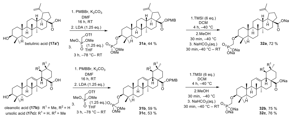
Scheme 6. Synthesis and demethylation of PMB-protected PCT derivatives 32a-c .
