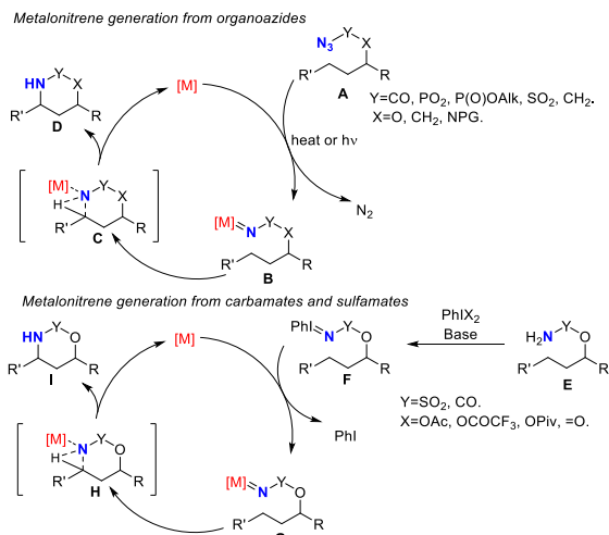
Scheme 12. Mechanisms of metalonitrene generation and following insertion in the C-H bond.
