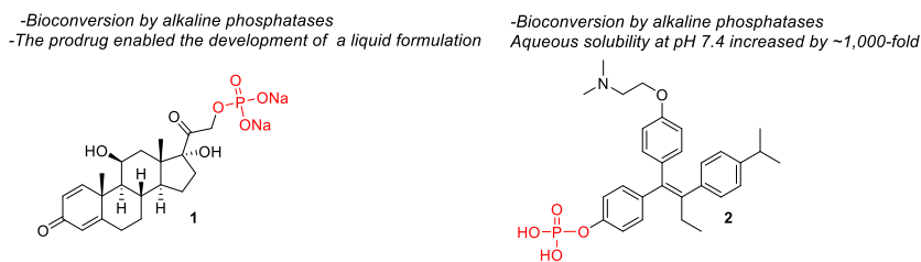
Fig. 3. Water-soluble prodrugs of prednisolone and miproxiifene.
