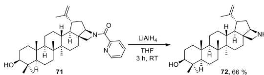
Scheme 19. Synthesis of unprotected azetidine 72 .
